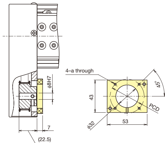
Motor bracket (detail) (symbol: A, B)
