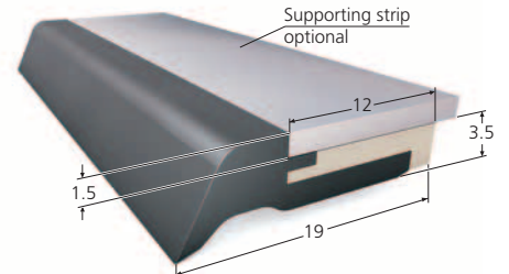
■ Wiper type MA 12
