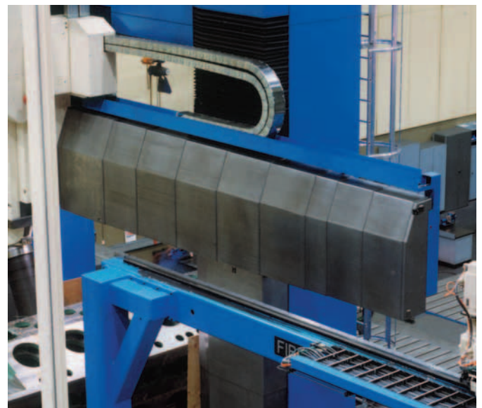
■ Cross-beam cover at a milling machine
