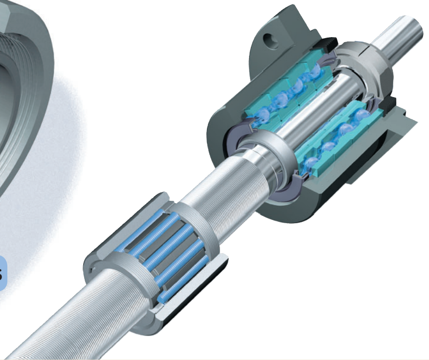
Recirculating roller screws
