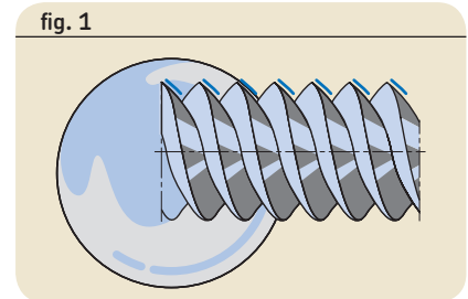
Threaded rollers are the basis of SR/BR/TR/PR planetary roller screws.
