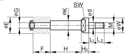
Fig. 5: TSP - Quill with nut (MU)
