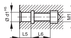
Close-fit hole for type 2 and 3
